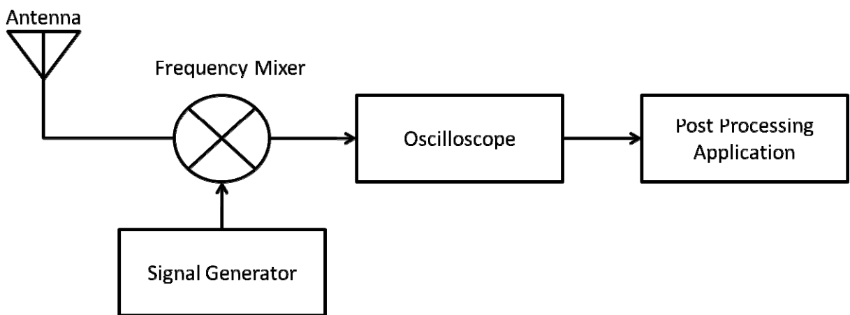
Figure 2 — Receiving setup
